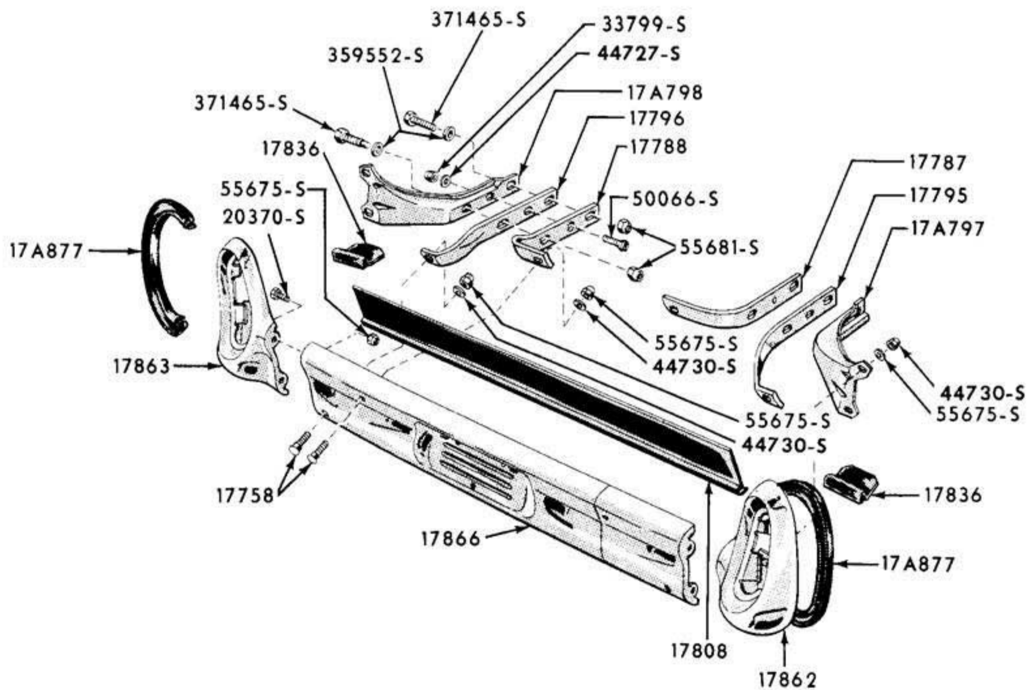
FRONT BUMPER and RELATED PARTS
