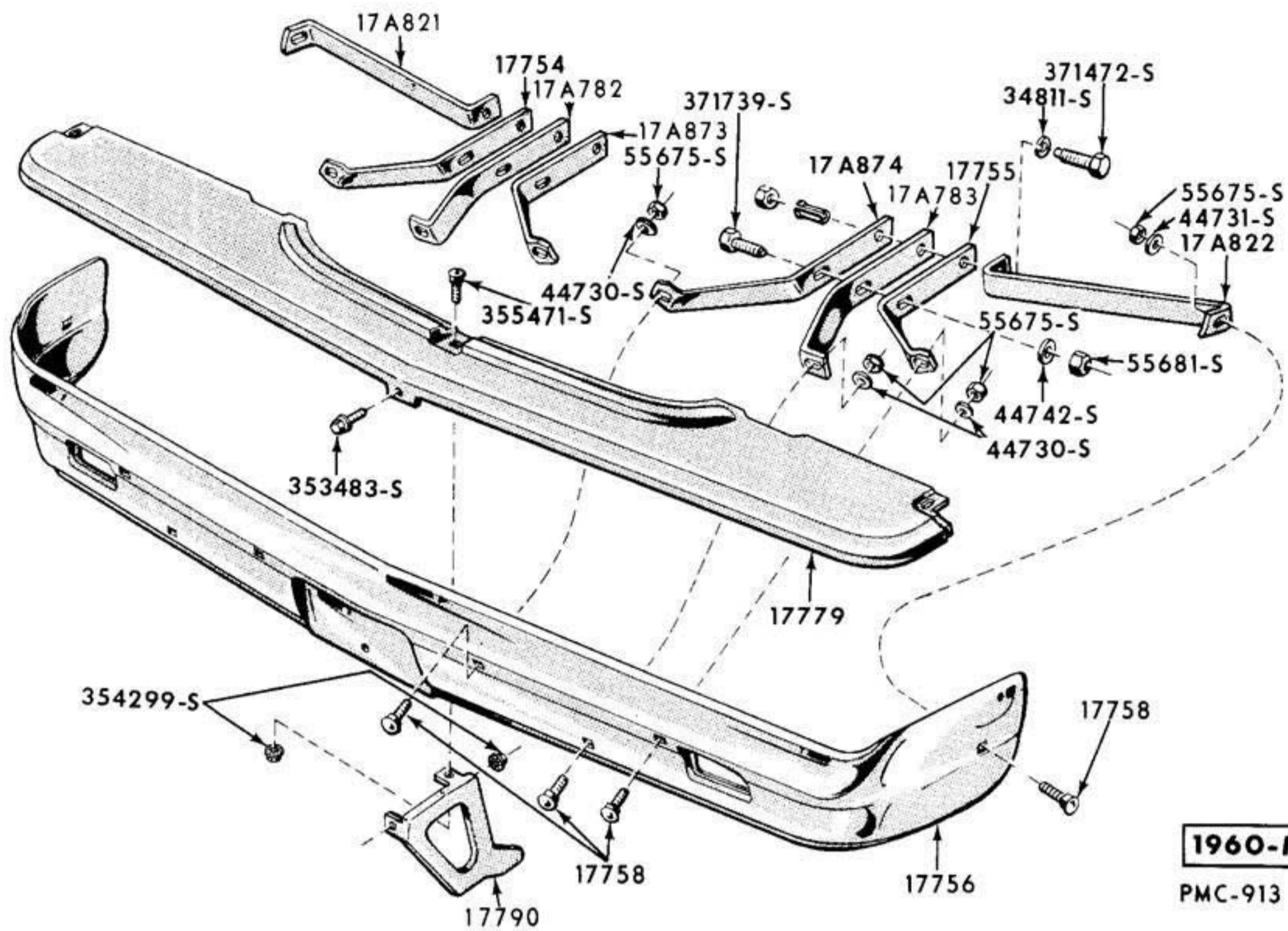
FRONT BUMPER and RELATED PARTS
