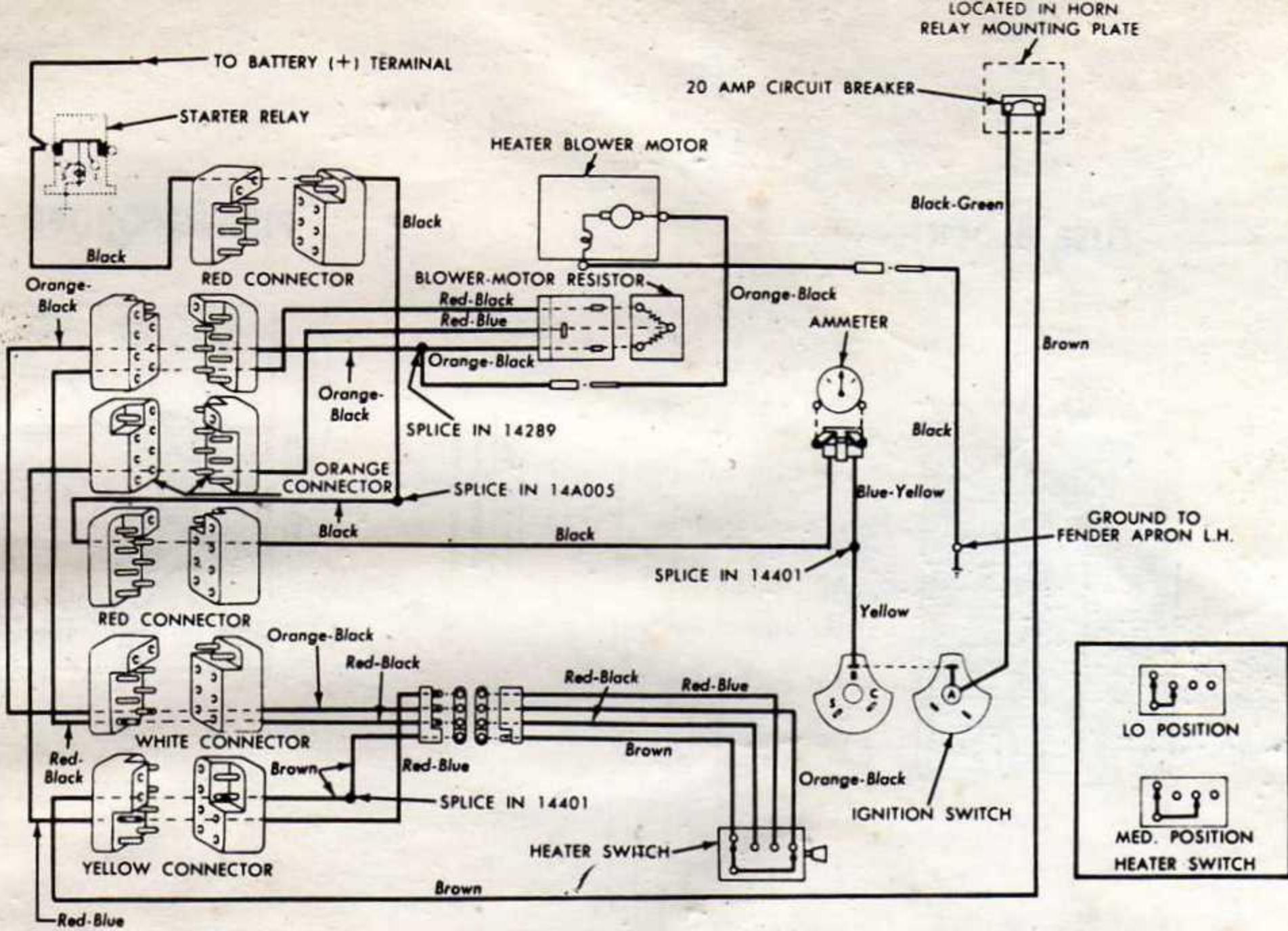
Heater & Blower Motor Circuit . . 1964
