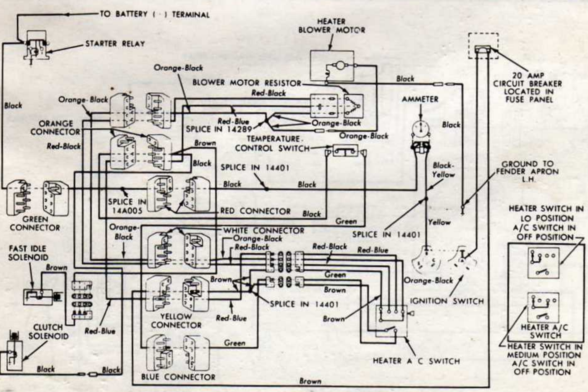
Air Conditioner & Heater Circuit . . 1964
