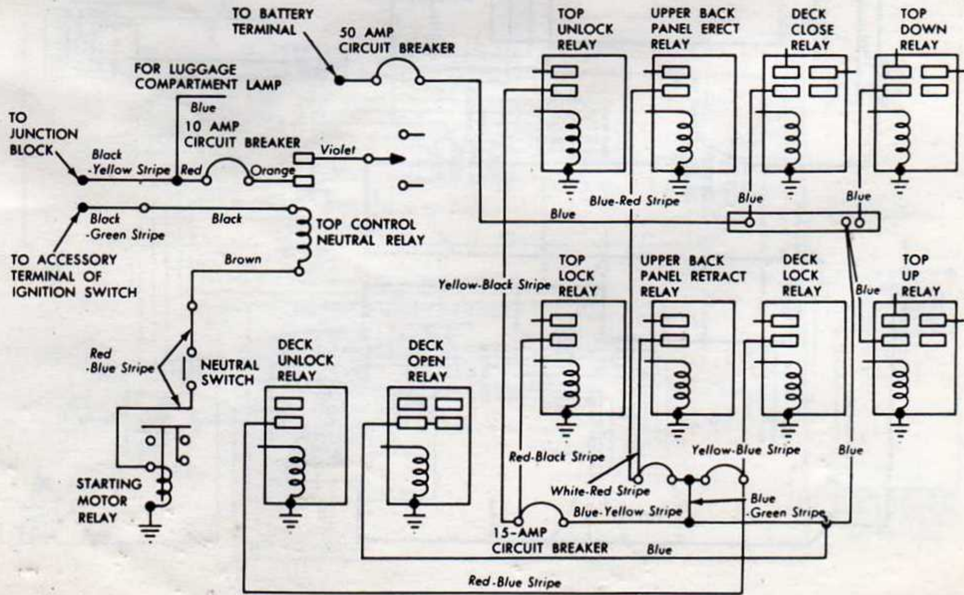
Convertible Top Control & Power Feed Circuit . . 1964
