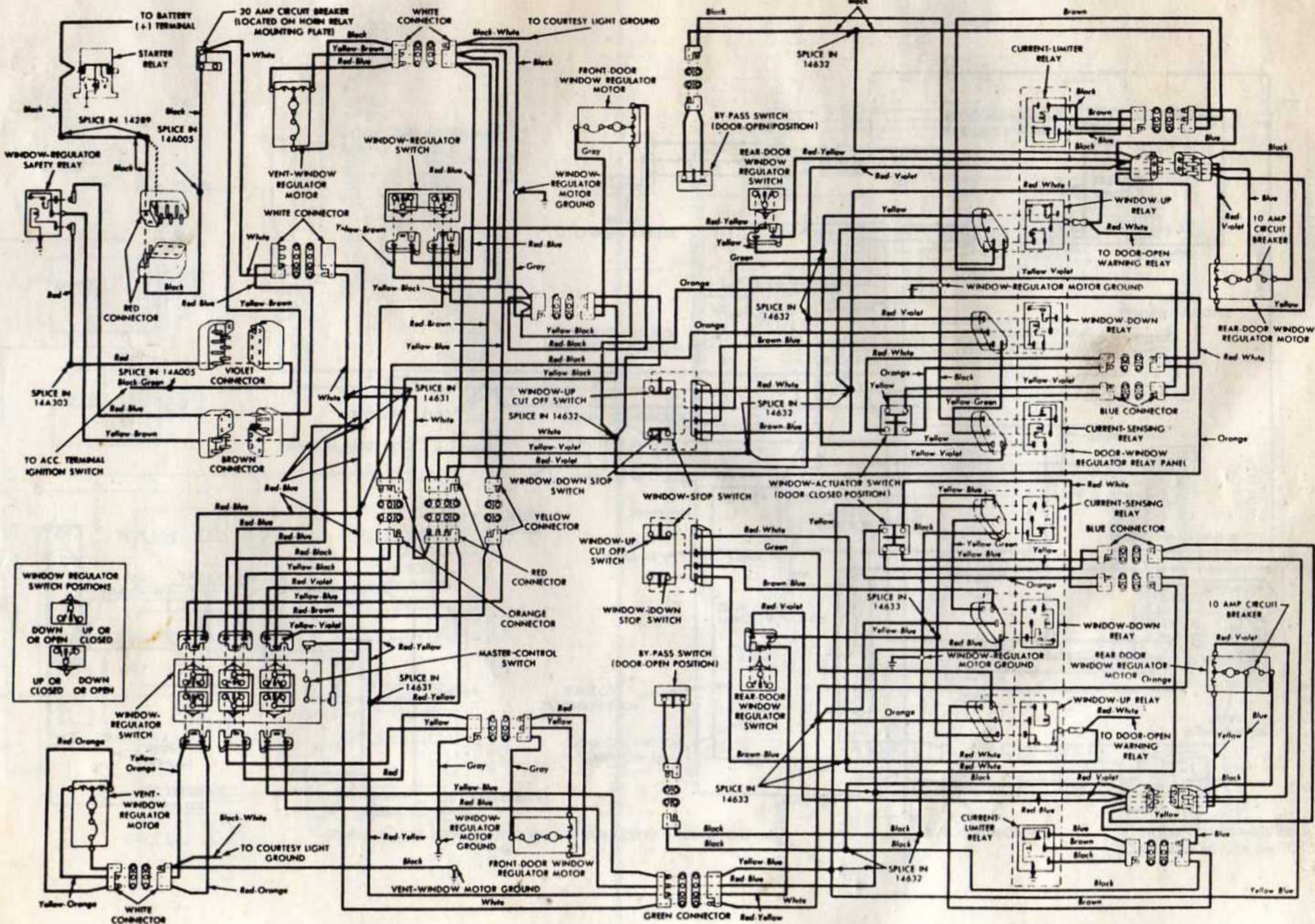
Power Window Circuit . . 1964 Sedans (Front window circuits apply to convertible)
