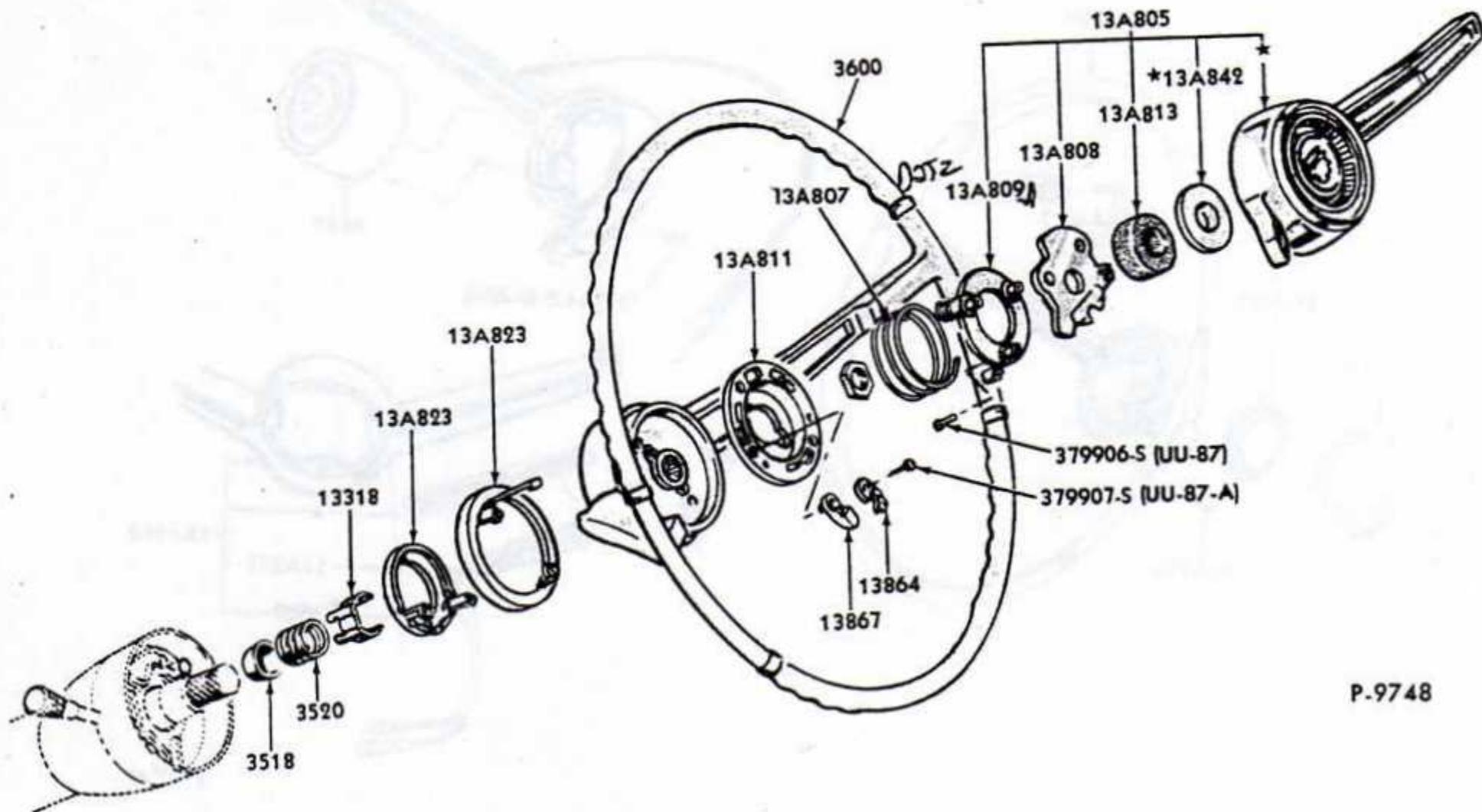
HORN RING and STEERING WHEEL 1965 COMET
