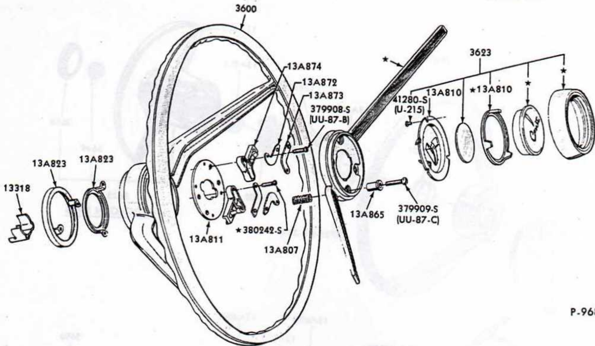
HORN RING and STEERING WHEEL 1966 COMET
