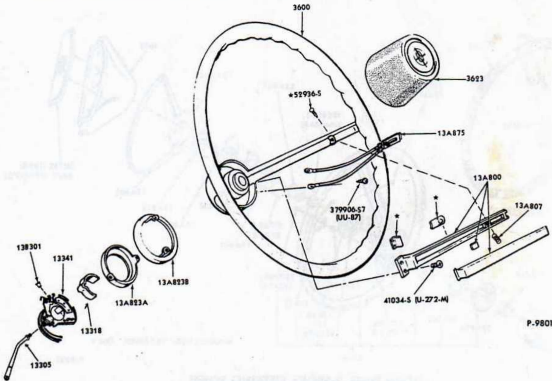
HORN BUTTON and STEERING WHEEL 1967 LINCOLN
