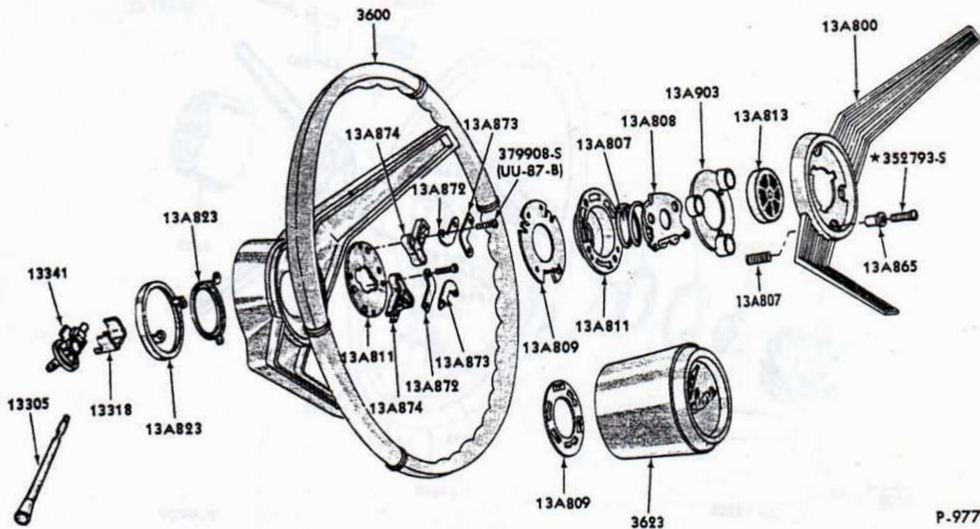
HORN RING and STEERING WHEEL 1967 COMET
